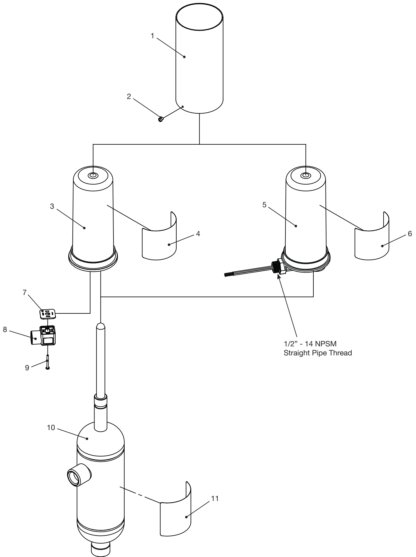
LLSS Exploded View
