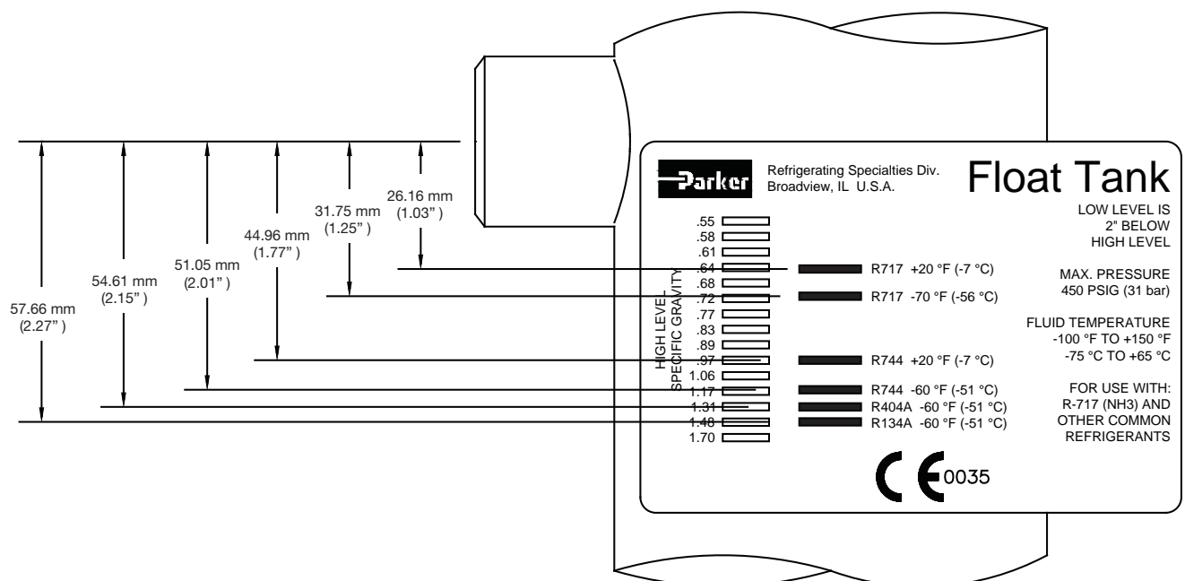
Float Tank Nameplate and Refrigerant Level Location
